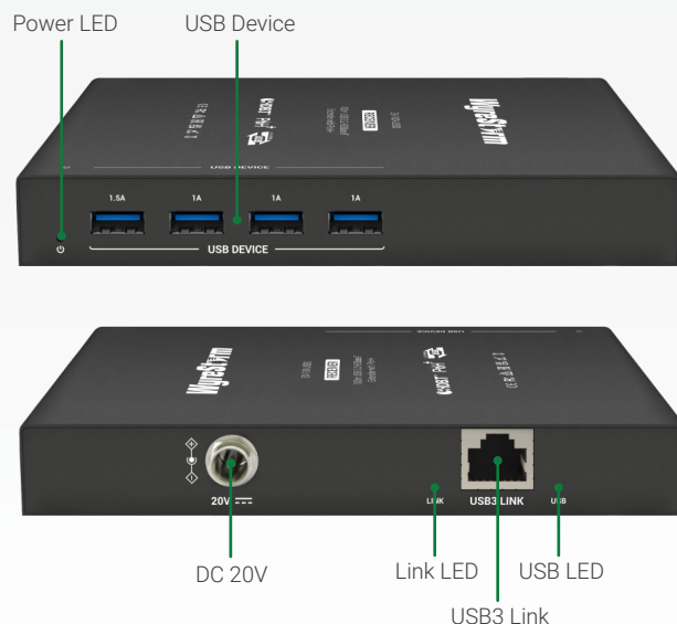
EX-100-IW-USBC (Rear)
