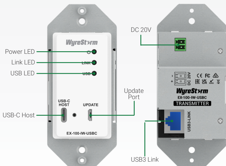
EX-100-IW-USBC (Front)
