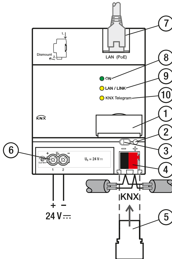
Fig. 3: Connection diagram
