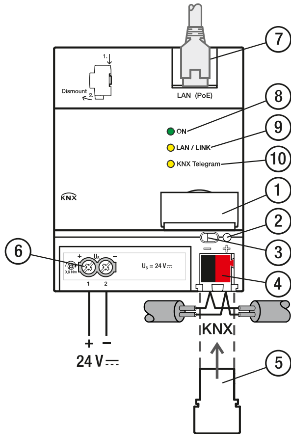
Fig. 6: Connection diagram
