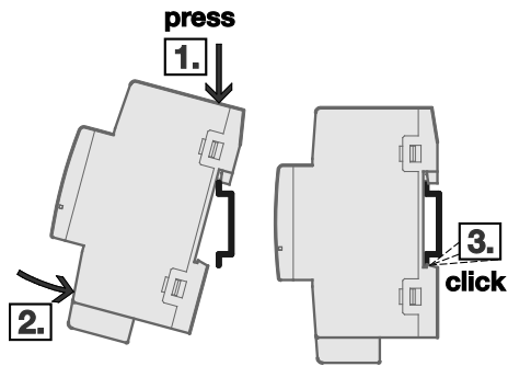
Fig. 8: Mounting
