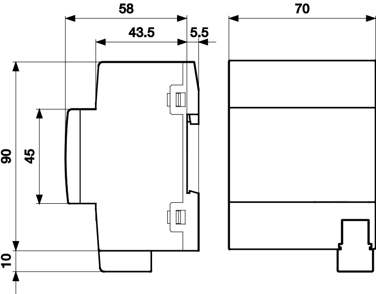
Fig. 5: Dimension drawing
