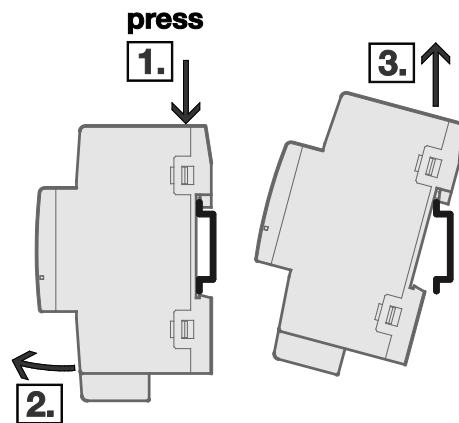
Fig. 10: Removal
